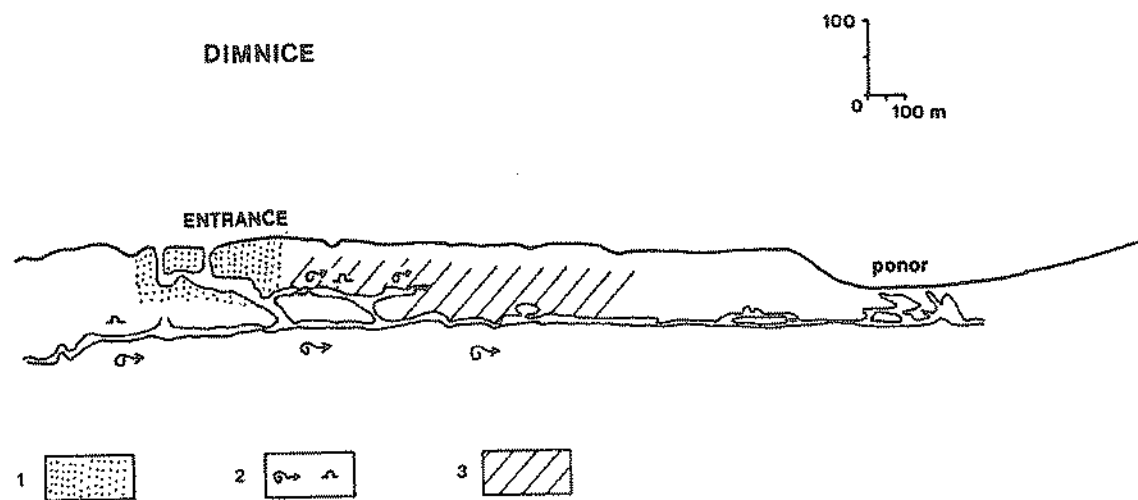
Fig. 1b: Longitudinal cross-section with rocky relief. 1. traces of water trickling down, moisture condensation and freezing, 2. traces of water flow, 3. along-sediment rocky features. Sl. 1b: Vzdolžni prerez jame s skalnim reliefom. 1 sledi polzeče vode, kondenzacije vlage in zmrzali, 2 sledi vodnih tokov, 3 obnaplavinske skalne oblike.
