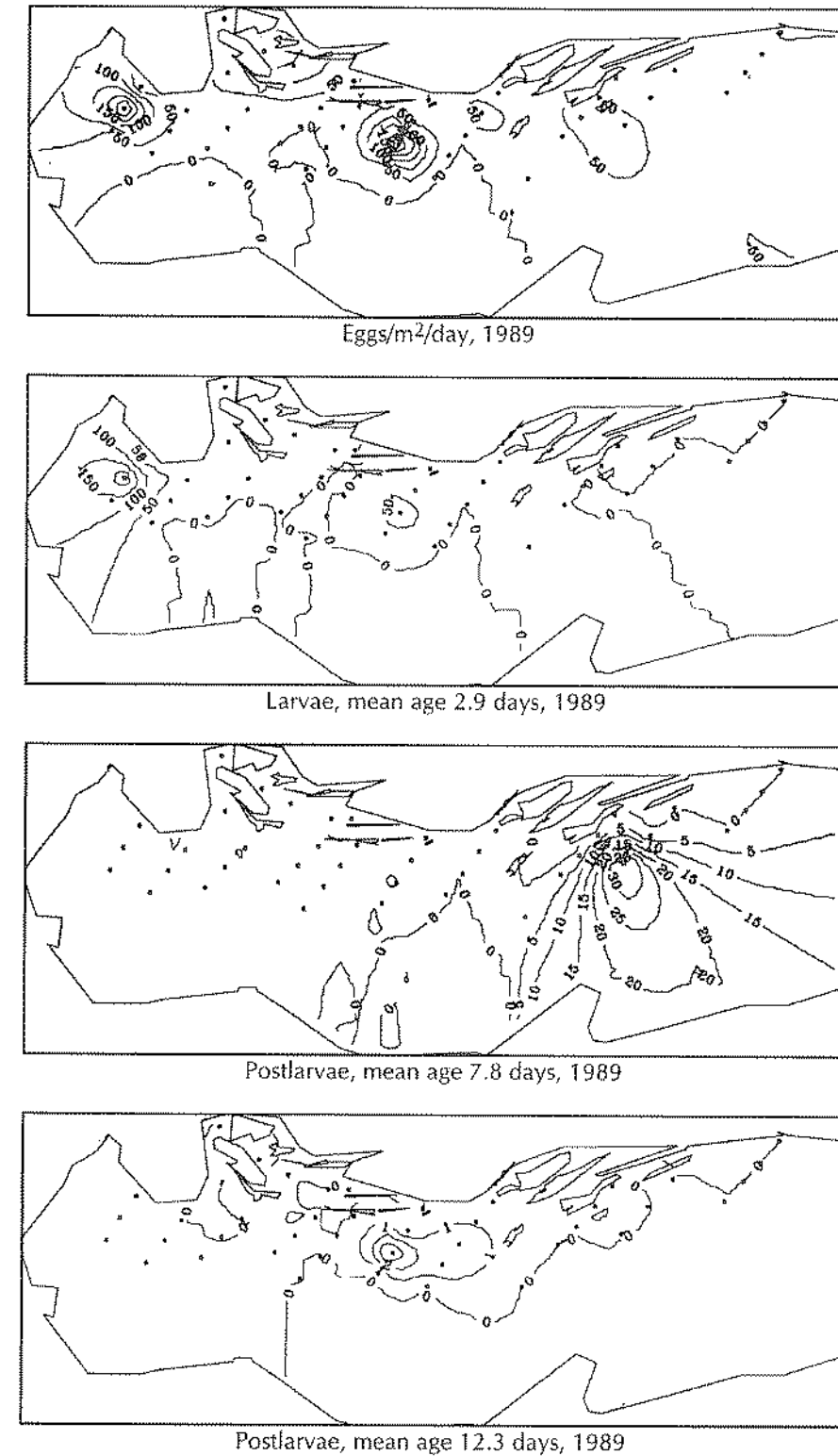
Fig. 6: Horizontal distribution of anchovy eggs, larvae, and postlarvae ( N/m^2/day ) along the Eastern Adriatic coast in August, 1989.
