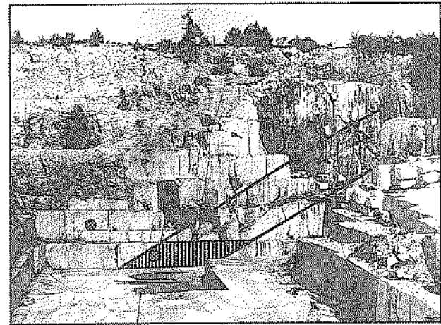
Sl. 2: Položaj raziskanih vzorcev rudistnega apnenca iz najnižje etaže kamnoloma Lipica I. Vrisana sta dva nivoja pogostnega pojavljanja vrste Keramosphaerina tergestina (Stache). Fig. 2: Position of studied samples of the rudist limestone from the lowest bench of the Lipica I quarry. Two levels of frequent appearance of species Keramosphaerina tergestina (Stache) are marked.
