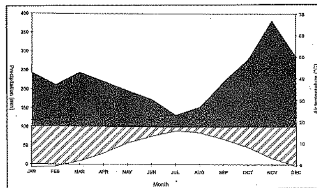
Fig. 1: Climatic Diagram (Zupančič, 1995; Mekinda-Majaron, 1995) - Gomance 1961-1990, according to Walter et al. (1964).
