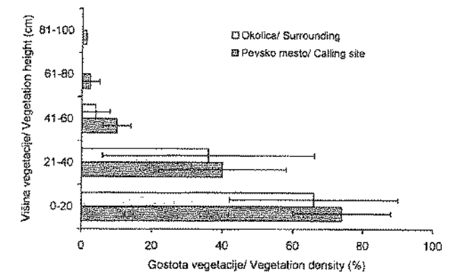
Fig. 2: Vegetation density in 20 cm-layers (mean values and standard errors), estimated from a distance of 0.5 m at the calling site as well as in four points in the surrounding; Kobariski Stol, June 16 th , 1994.
