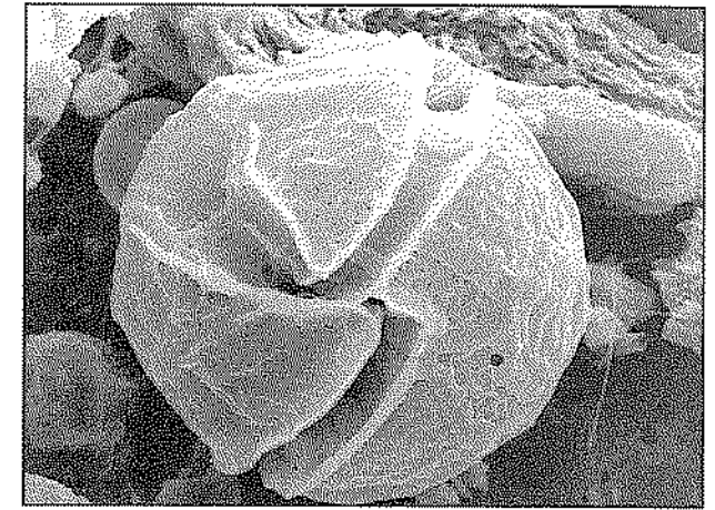
Fig. 5: Scanning electron micrograph of Alexandrium sp. (presumably related to A. acatenella ) from the southeastern part of the Gulf of Trieste.
