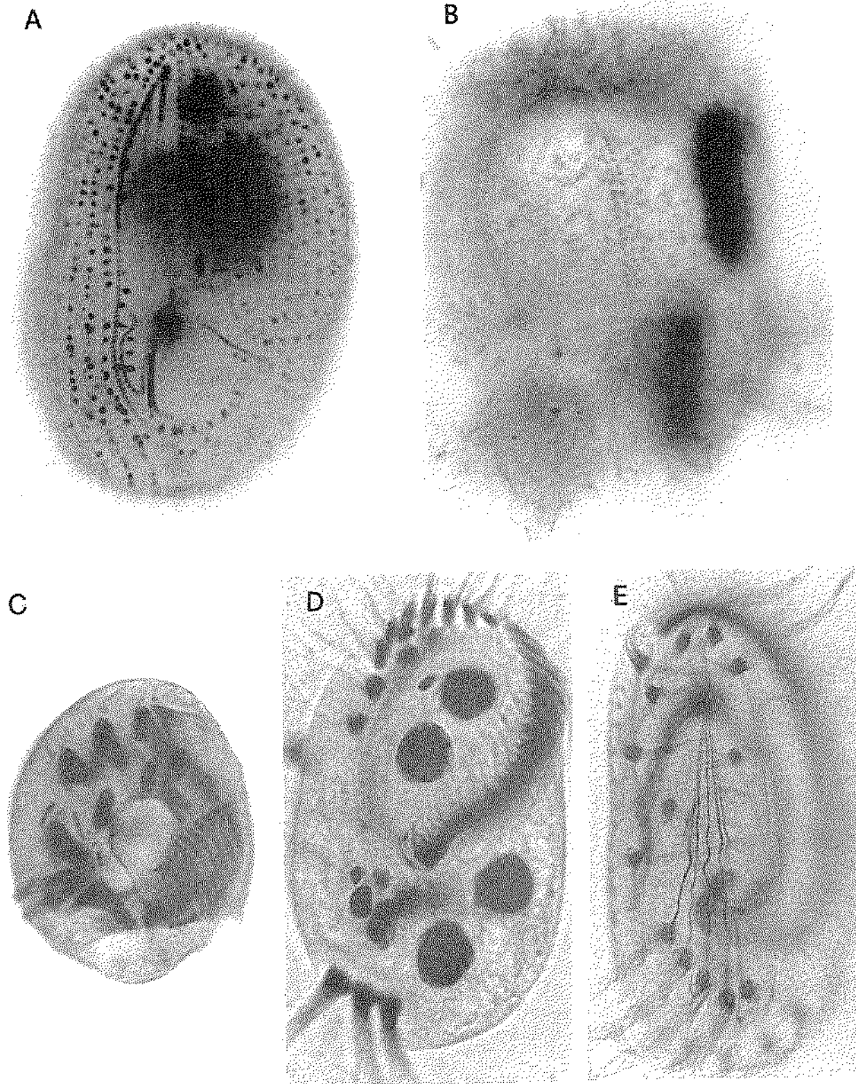
Fig. 5: Micrographs of protargol-impregnated specimens. A: Pleuronema coronatum , ventral view, 1120x; B: Uronychia transfuga , dorsal view, 1280x; C: Aspidisca sedigita , ventral view, 1280x; D: Diophrys appendiculata , ventral view, 1280x; E: Euplotes vannus , ventral view, 960x.
