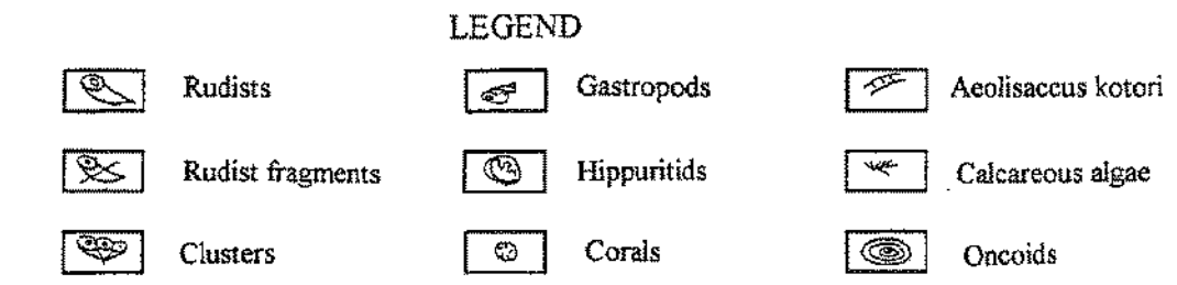
Fig. 2: Stratigraphic sequence of Slivia. Sl. 2: Stratigrafski stolpec Slivja.
