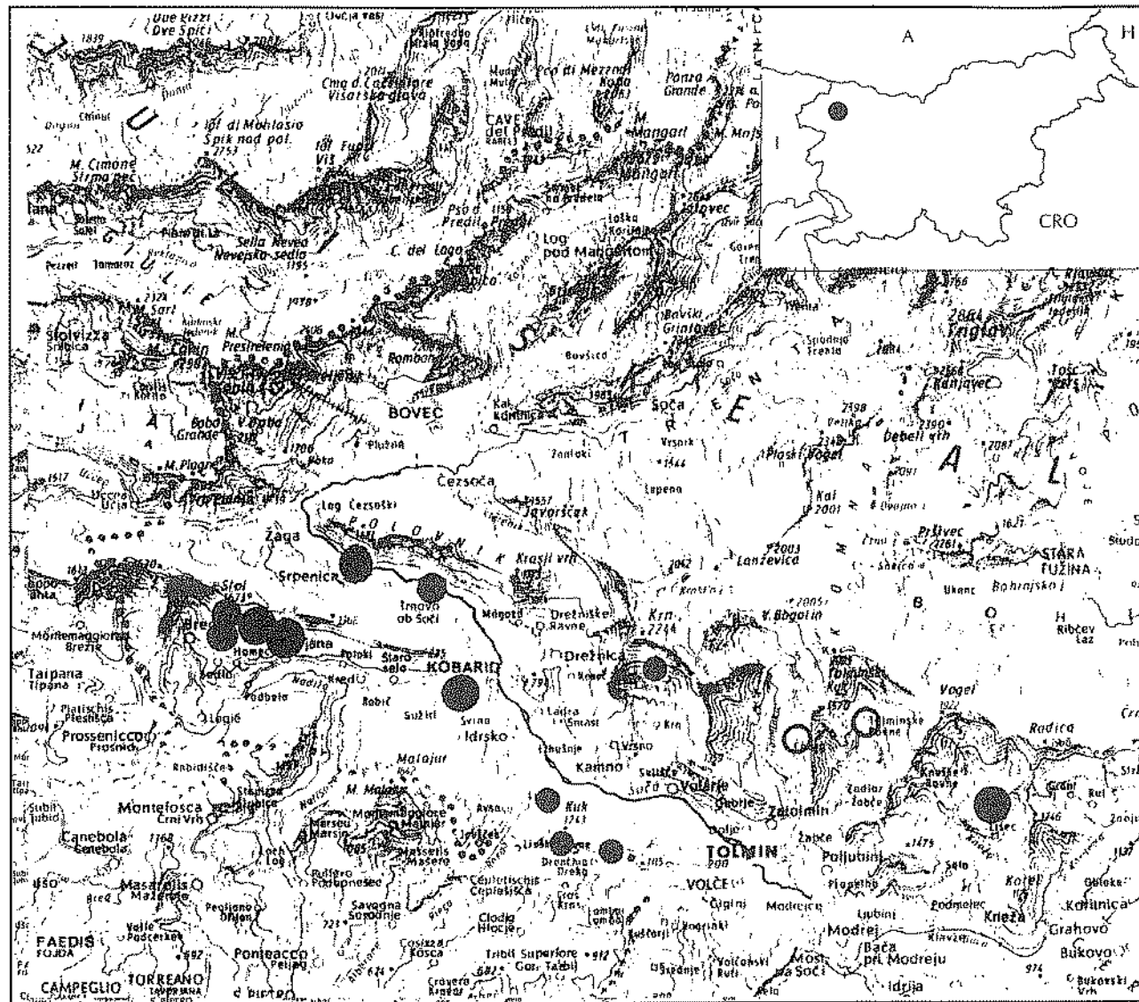
Fig. 1: Distribution of the Corn crake ( Crex crex ) at the upper Soča basin. Dot size app. reflects the number of calling males. Empty circles indicate abandoned sites.
