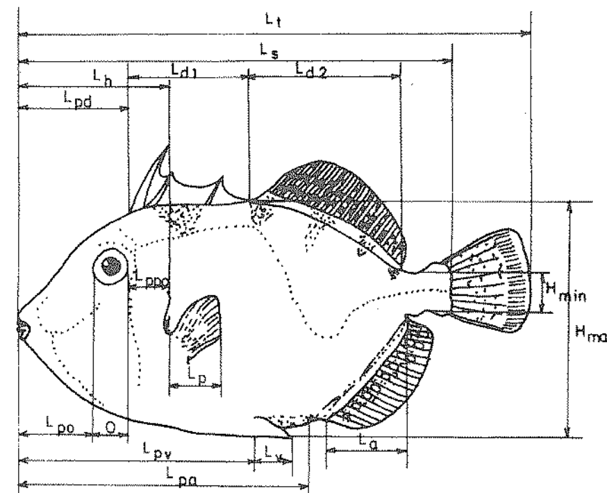
Fig. 2: Body measurements of Balistes carolinensis fingerlings. L t - total length; L s - standard length; L pd - predorsal length; L p - preventral length; L h - head length; O - eye diameter, L po - preorbital length; L ppo - postorbital length; L d1 - first dorsal fin length; L d2 - second dorsal fin length; L p - pectoral fin length; L v - ventral fin length; L a - anal fin length; L pa - preanal length; H min - minimal body depth; H max - maximal body depth at dorsal fin.
