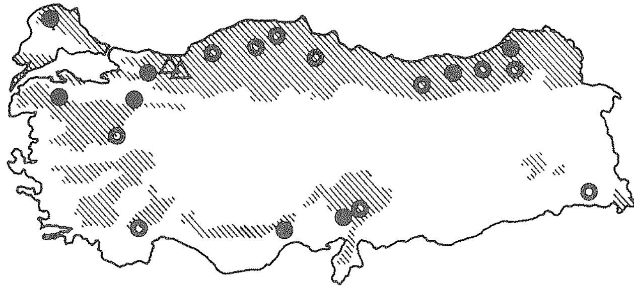
Fig. 1: Distribution of the wild cat Felis silvestris in Turkey. Tentative range, as proposed by Turan (1984), is shaded. Given are also published records (dots) as well as the localities obtained through inquiry (circles). The origin of the two specimens, reported in this communication, is indicated by triangles.
