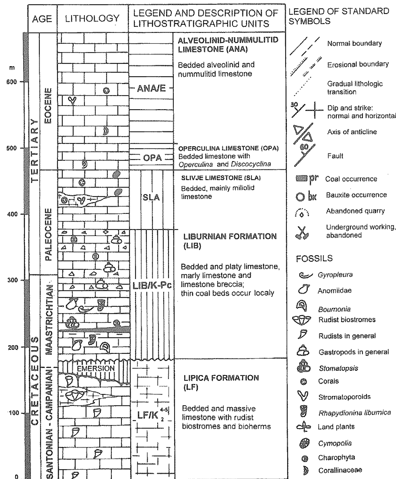
Sl. 2: Litostratigrafsko zaporedje plasti na ozemlju avtocestnega odseka Divača - Kozina z legendo k stolpcu in geološki karti. Fig. 2: Lithostratigraphic succession of the beds in the Divača - Kozina motorway section with legend to the column and geological map.
