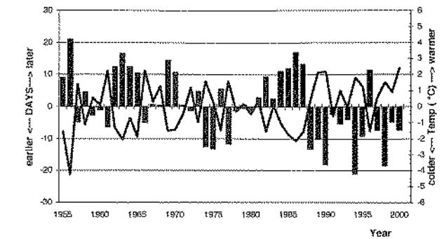
Fig. 3: Early-spring flowering index and air temperatures with deviations from the long-term means (1955-2000). Vertical bars represent the annual early-spring indexes (the mean of flowering dates for: Betula pendula , Taraxacum officinale , Salix caprea , Corylus avellana and Galanthus nivalis ) expressed as deviations in days from the mean value. The line represents the annual deviations of temperature (°C) from the spring mean temperature (February-April).
