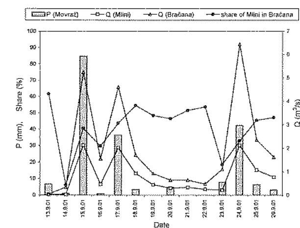
Fig. 3: The share of Mlini springs in the total discharge of the Bračana stream.
