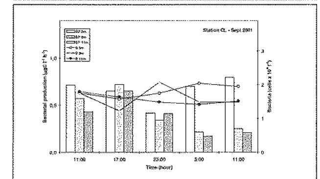
Fig. 3: Bacterial abundance and bacterial production in the water column during 24-hour cycle at the station near the fish cages (station SL) and the station 200m away from the cages (station CL) in September 2001.
