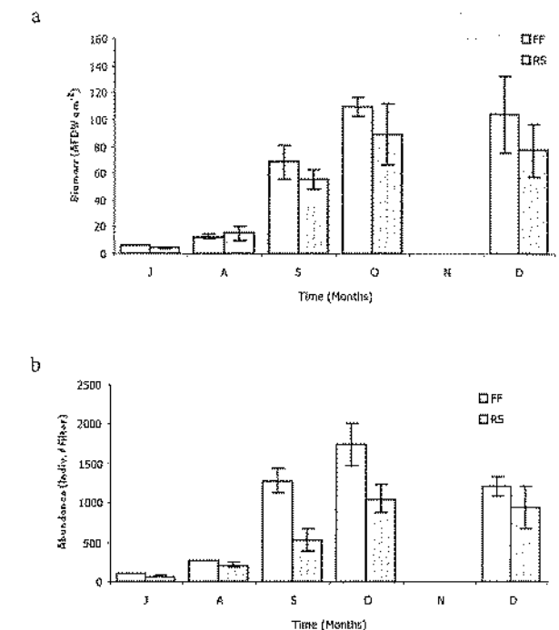
Fig. 1. Biomass (AFDW g m -2 ) (a) and abundance (No. individuals cylinder -1 ) (b) of macrofauna on mesh cylinders at the fish farm (FF) and reference site (RS) in the Lynne of Lorne, west Scotland at the monthly sampling periods (July – December 2001). Mean values ( n = 4 ) and standard deviations (error bars) are shown. Sl. 1: Biomasa (AFDW g m -2 ) (a) in abunanca (No. osebkov cilinder -1 ) (b) makrofavne na biofiltrih ob ribogojnici (FF) in na referenčni postaji (RS) v Lynne of Lorne (zahodna Škotska) na posameznih mesečnih vzorčevanjih (Julij – December 2001). Prikazane so povprečne vrednosti ( n = 4 ) in standardne deviacije.
