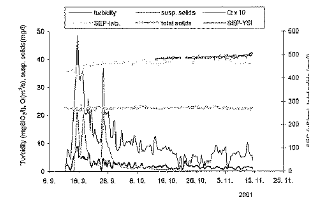
Fig. 4: Mlini spring: measurements of turbidity, total suspended solids, total solids and conductivity – SEC in autumn 2001 (5-term smoothing used for the measuring of turbidity and suspended matter).
