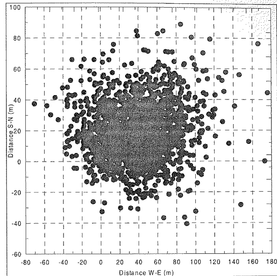
Fig. 3: Simulated distribution of faecal particles on the seabed using trajectories data from the currents measured between April 19 and June 21. The sinking velocity was 0.64 \pm 0.05 \text{ cm/s} .
