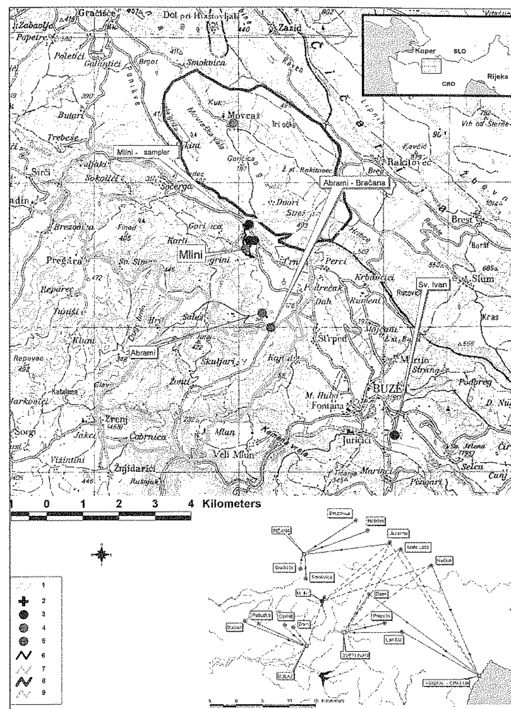
Fig. 1: Location map and the presentation of results of tracing tests in the wider area of Mlini springs: 1 – state border; 2 – automatic water sampler; 3 – spring; 4 – precipitation station; 5 – hydrological station; 6 – hydrographic network; 7 – surface watershed of the Bračana; 8 – hydrogeological watershed of Mlini spring; 9 – surface watershed of the Bračana – Abrami station.
