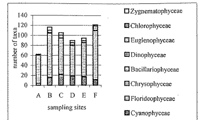
Fig. 2: Algal community structure in the river Dragonja and its tributary Pinjevec during the years 1998, 1999 and 2000 (A – source, B – Škrline, C – pool, D – slow current, E – strong current, F – estuary).
