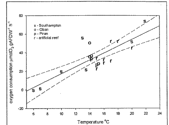
Fig. 2: Oxygen consumption by different communities plotted against incubation temperature: experimental biofilters from Southampton, Oban and Piran and concrete artificial reef blocks from Poole Bay (Collins et al. , 2002), showing a linear regression line with 95% confidence intervals.
