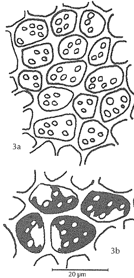
Fig. 3: Cell arrangement (a) and the chloroplast structure with pyrenoids (b).
