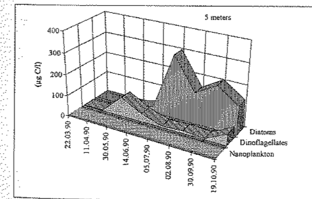
Fig. 5: Relationship between Particulate Phytoplankton Carbon (PPC - µgC/l) on the left and the abundance of phytoplankton cells (cells/l) on the right at the station 1 (surface and 5 meters).
