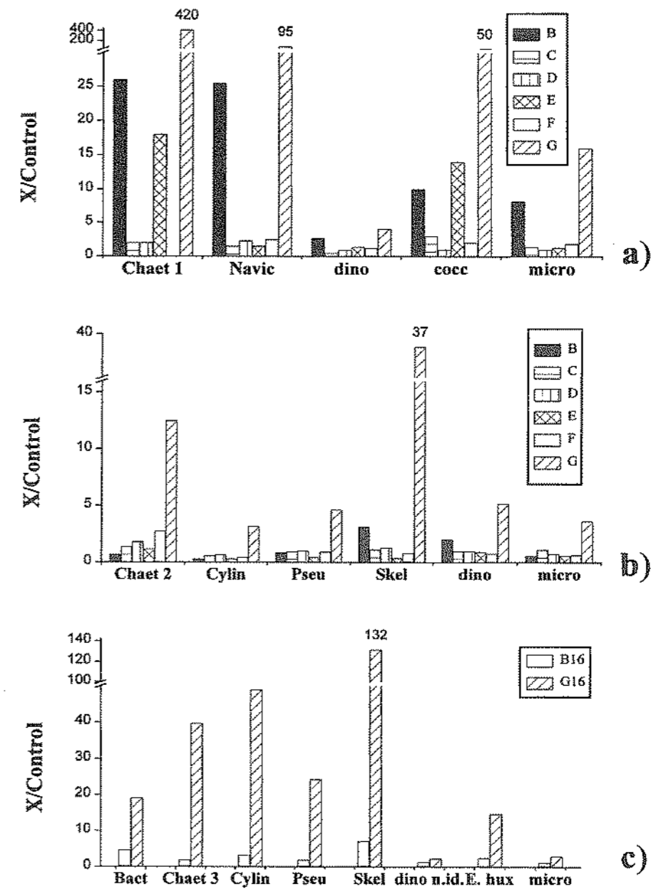
Fig. 3: Ratios between the abundance of dominant phytoplankton species/groups in different treatments (X) and the respective abundance in control conditions on day 6 during PALEX experiments 1 (a), 2 (b) and 3 (c). Only data for assemblage collected at the depth of fluorescence maximum (16 m) are shown for PALEX 3.
