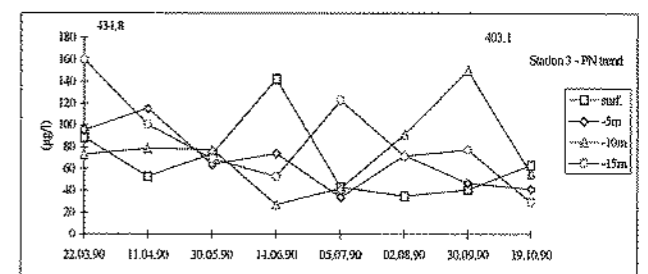
Fig. 3: Particulate Nitrogen (PN) at the stations 1, 2 and 3.
