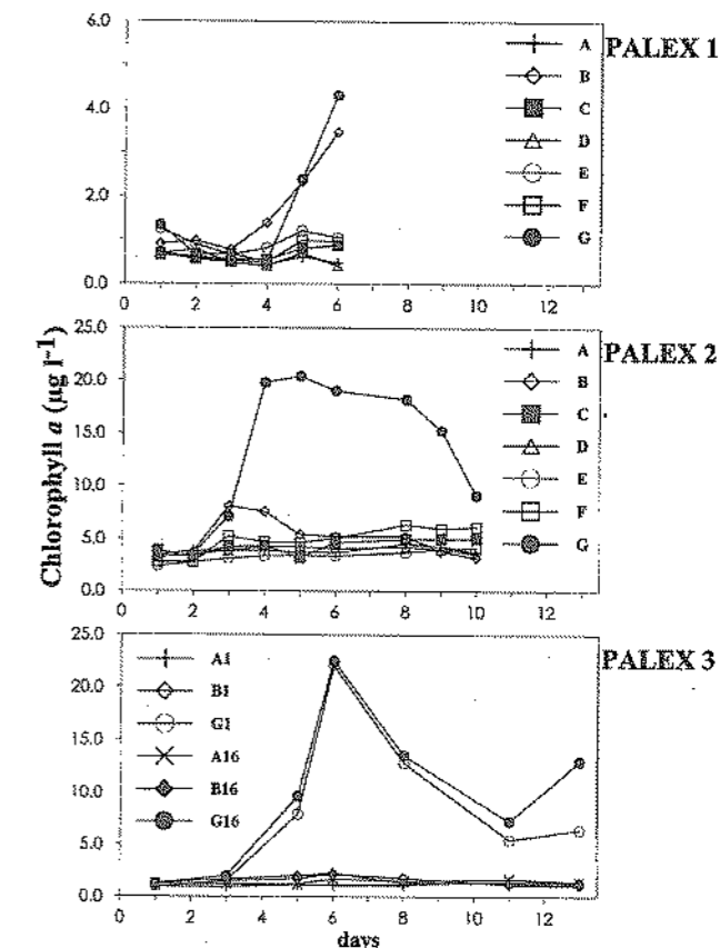
Fig. 1: Chlorophyll a biomass in different nutrient treatments during PALEX experiments 1 (27 June - 2 July 1994), 2 (3-12 April 1995) and 3 (22 March - 3 April 1996).
